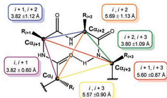
Figure 2. Mean and standard deviations of the C\alpha distances taken from a set of 10 245 \beta -turns in the PDB.
