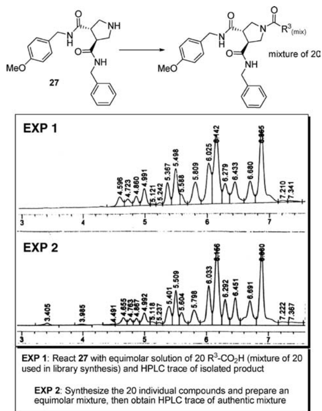
Figure 9. HPLC comparison of library (EXP 1) and authentic (EXP 2) equimolar mixture of the final 20 compounds derived from 27 . HPLC conditions: linear gradient, 0–90% MeCN in H 2 O over 7 min and then 90% MeCN for 10 min at a flow rate of 0.75 mL/min.
