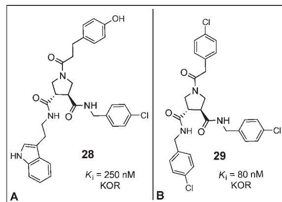
Figure 14. Chemical structures of compounds with the highest affinity for KOR from the Trp/Phe(4Cl) series ( 28 ) and the Phe(4Cl)/Phe(4Cl) series ( 29 ).
