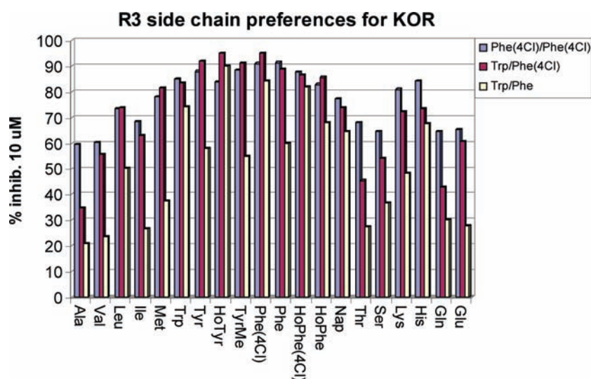
Figure 15. Screening results (% inhibition at 10 \mu\text{M} ) for the three series of deconvolution compounds against KOR (versus [ ^3\text{H} ]U69593).
