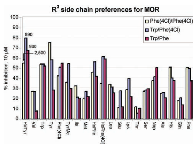
Figure 12. Screening results (% inhibition at 10\ \mu\text{M} ) for the three series of deconvolution compounds against MOR along with measured K_i values (nM) (versus [^3\text{H}]\text{DAMGO} ).
