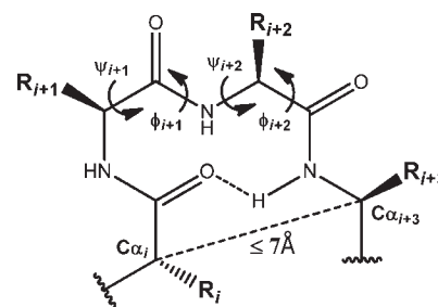
Figure 1. Schematic diagram of a \beta -turn.
