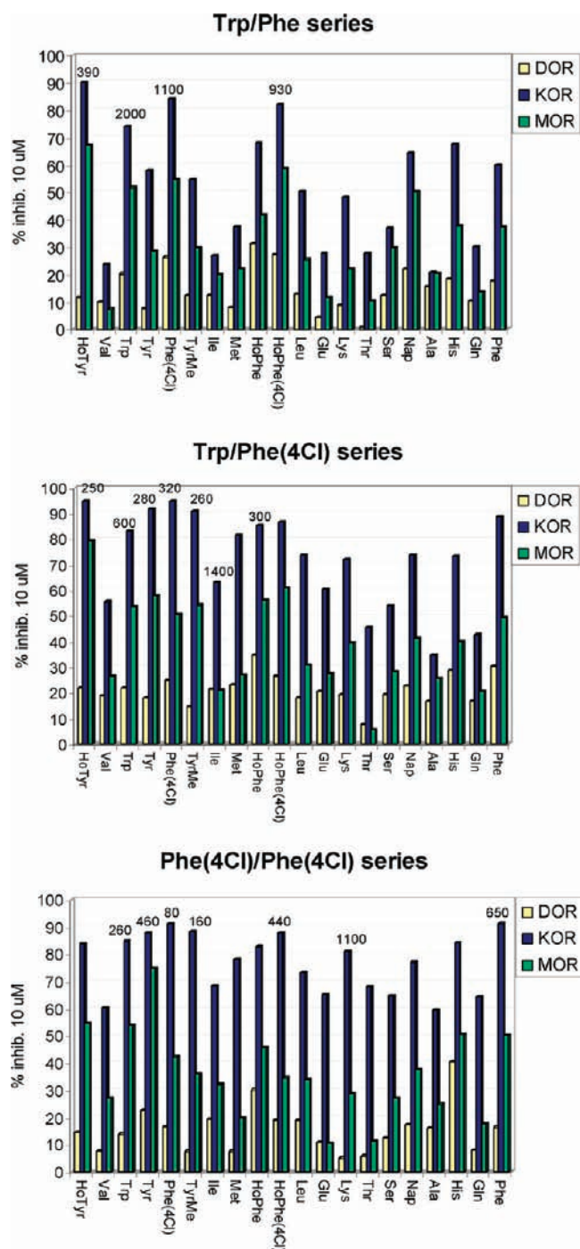
Figure 13. Screening results (% inhibition at 10 \mu M) for the three series of deconvolution compounds against KOR (versus [ 3 H]U69593), MOR (versus [ 3 H]DAMGO), and DOR (versus [ 3 H]DADLE) along with measured K_i values (nM) against KOR.
