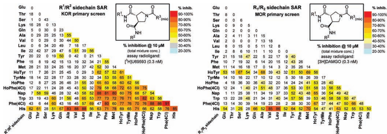
Figure 10. (A) % inhibition of [^3\text{H}]\text{U69593} binding for the indicated \text{R}^1/\text{R}^2 side-chain combinations in the screening of the 210 mixtures against the KOR. (B) % inhibition of [^3\text{H}]\text{DAMGO} binding for the indicated \text{R}^1/\text{R}^2 side-chain combinations in the screening of the 210 mixtures against the MOR.
