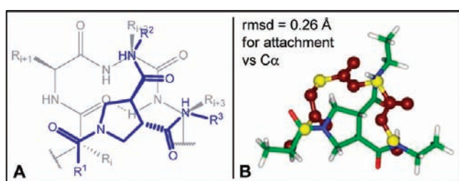
Figure 4. (A) Overlay of a potential mode of \beta -turn mimicry by a trisubstituted trans -pyrrolidine-3,4-dicarboxamide. (B) Overlay and calculated rmsd value for attachment of the three substituted centers of the template with three \alpha -carbons in a type-I \beta -turn.
