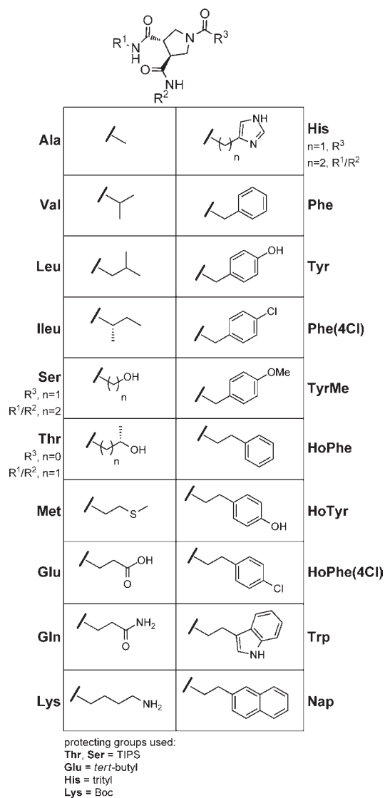
Figure 7. The 20 groups used in the synthesis of the \beta -turn mimetic library.
