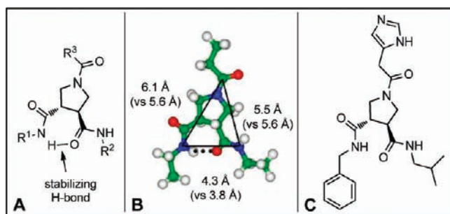
Figure 3. (A) The trans -pyrrolidine-3,4-dicarboxamide template. (B) Low-energy conformation and measured distances between substituted centers of a trans -pyrrolidine-3,4-dicarboxamide with ethyl substituents. (C) A trans -pyrrolidine-3,4-dicarboxamide substituted with groups representing the side chains of Leu, Phe, and His.
