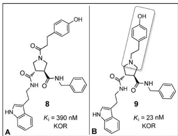
Figure 6. (A,B) Structures of high-affinity KOR-selective compounds 8 and 9 . The tyramine pharmacophore found in the “message” structure of opioid compounds and peptides is highlighted in (B).
